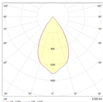
Downlight 14W 60°
