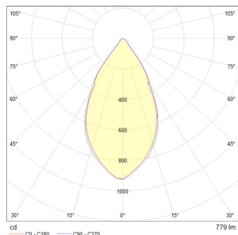
Downlight 9W 60°
