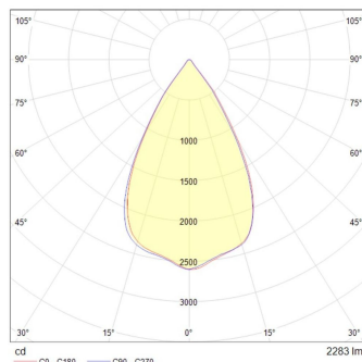
Downlight 28W 60°
