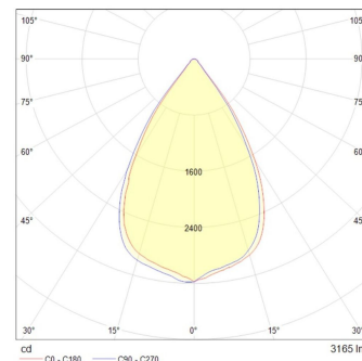
Downlight 34W 60°
